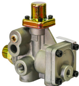
RDP3802 Spring Brake Valve SR3 65-75 PSi (ADR3802)
